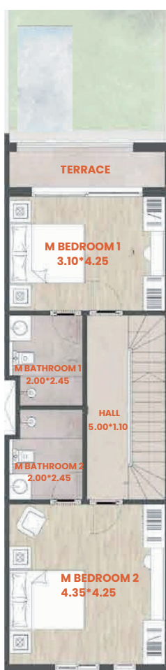
First Floor Plan
